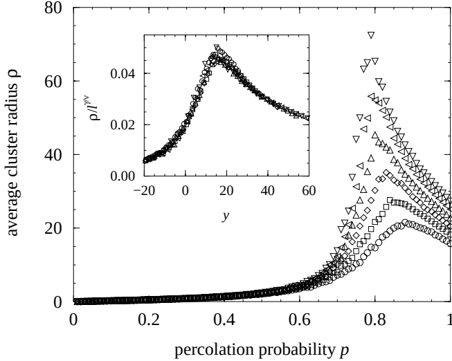
FIG. 8. Average cluster radius \rho as a function of the percolation probability p for site percolation on small-world graphs with k = 1 , \phi = 0.1 and L equal to a power from 512 up to 16 384 (circles, squares, diamonds, upward-pointing triangles, left-pointing triangles and downward-pointing triangles respectively). Each set of points is averaged over 100 realizations of the corresponding graph. Inset: the same data collapsed according to Eq. (33) with \nu = 0.59 , \gamma = 1.3 and p_c = 0.74 .
