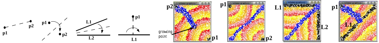
Figure 3: Huzita's axioms 1-4 and their implementation by the agents
