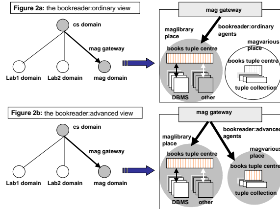
Fig. 2. An example of HiMAT interaction space
